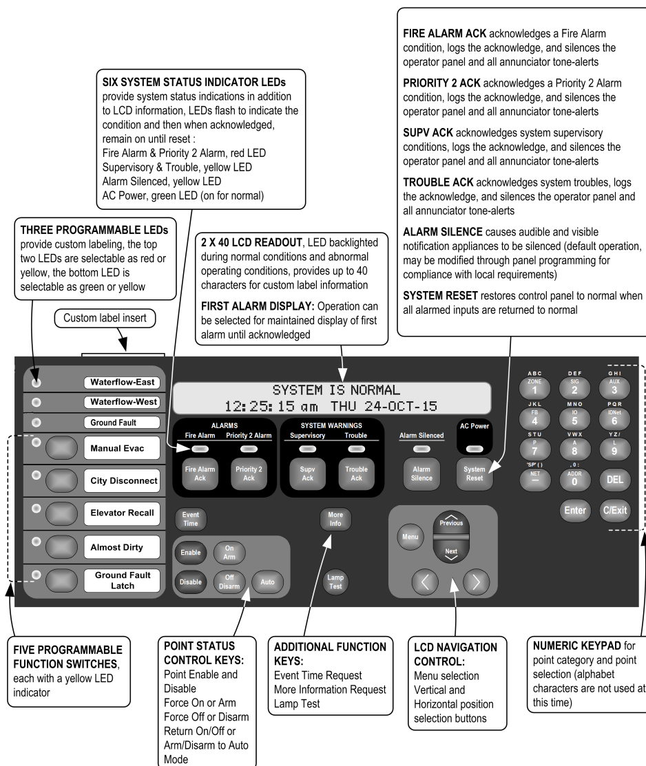
Figure 13: Operator Interface
