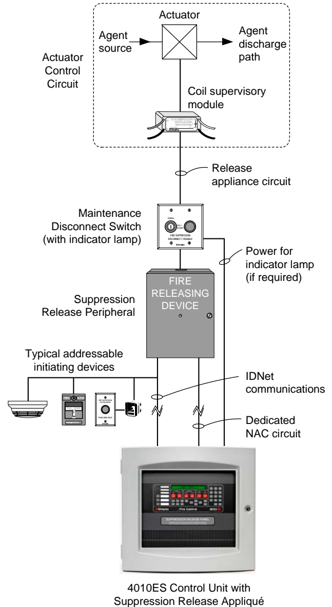
4010ES Release Control Simplified Block Diagram
